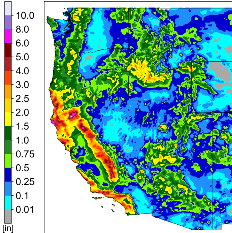
NWS Stage IV 72-h QPE Valid: 5 AM PT 16 Mar 2023
