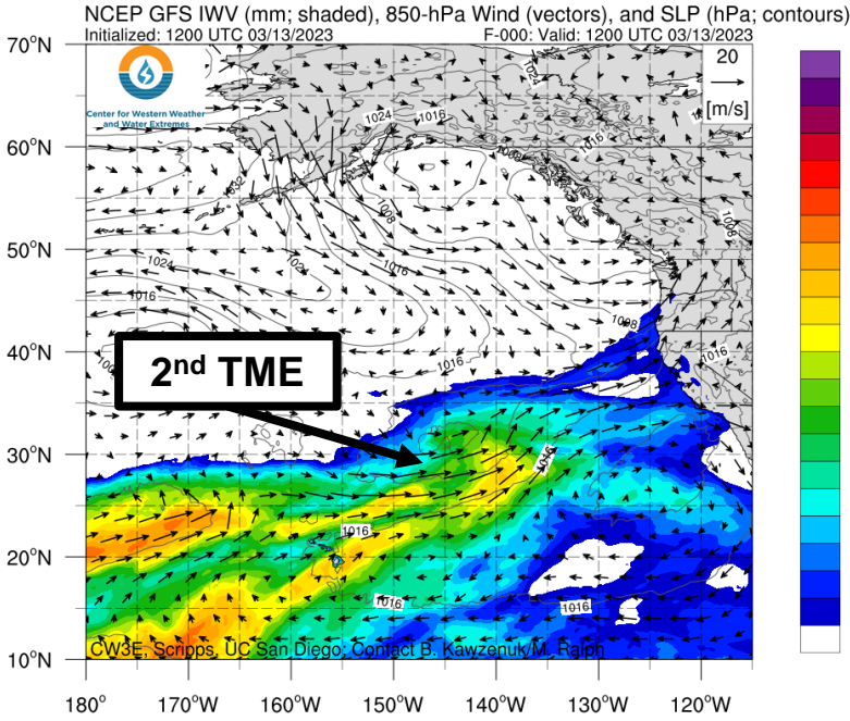
IWV and 850-hPa Wind
