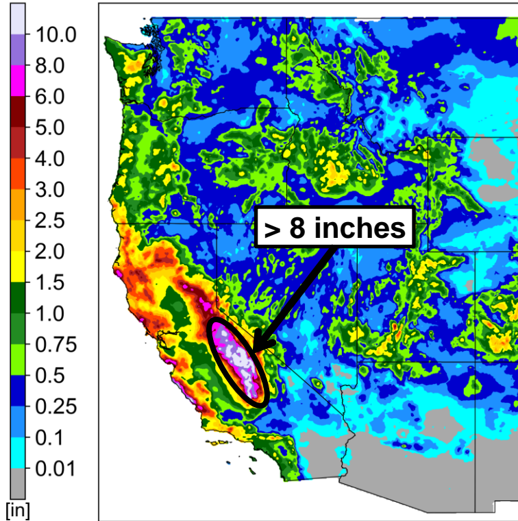
NWS Stage IV 72-h QPE Valid: 5 AM PT 12 Mar 2023
