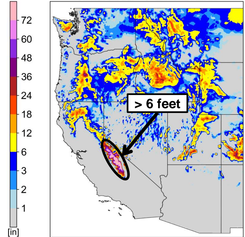
NWS 72-h Snowfall Analysis Valid: 5 AM PT 12 Mar 2023
