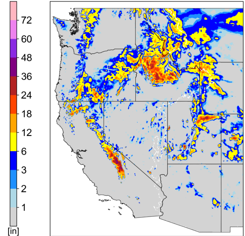
NWS 72-h Snowfall Analysis Valid: 5 AM PT 16 Mar 2023
